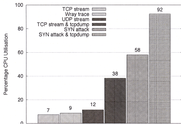
Figure 1. NETGEAR WG302 CPU utilisation under different conditions
